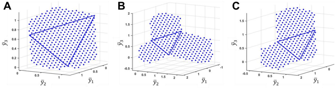
Figure 6.11: Different Utopian polygons in the 3-D objective space. They are controlled by the pseudo Nadir point ( \mathbf{y}^P ) (a), the Nadir point ( \mathbf{y}^N ) (b), and a mixed Nadir point ( \mathbf{y}^{P/N} = [y_1^N \ y_2^P \ y_3^N]^T ) (c), respectively.
