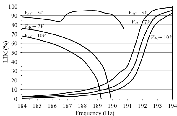
Figure 12. LIM integrity profiles to analyze the practical jump and pull-in dynamics.
