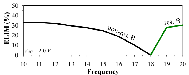
Fig. 5. ELIM integrity profiles for the initial condition of rest in the left well, at V_{AC} = 2.0 V .
